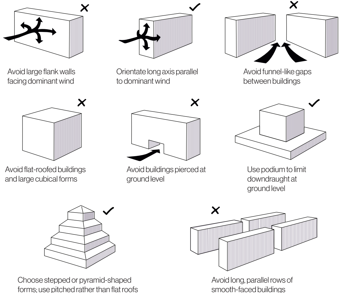
Figure 40: Reducing the wind sensitivity of buildings
