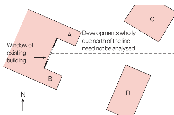
Figure 27: In analysing the sunlighting impact on the existing window, no check need be made for proposed extension A and new building C, as they lie within 90^\circ of due north of the window. Proposed extension B should be checked, as should new building D if it subtends more than 25^\circ to the horizontal, measured in section from the centre of the window
