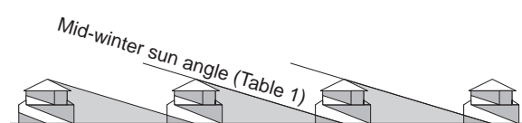
Figure 34: Passive solar homes at Giffard Park, Milton Keynes (top), the terraces at Giffard Park are carefully spaced to avoid winter overshadowing (below)
