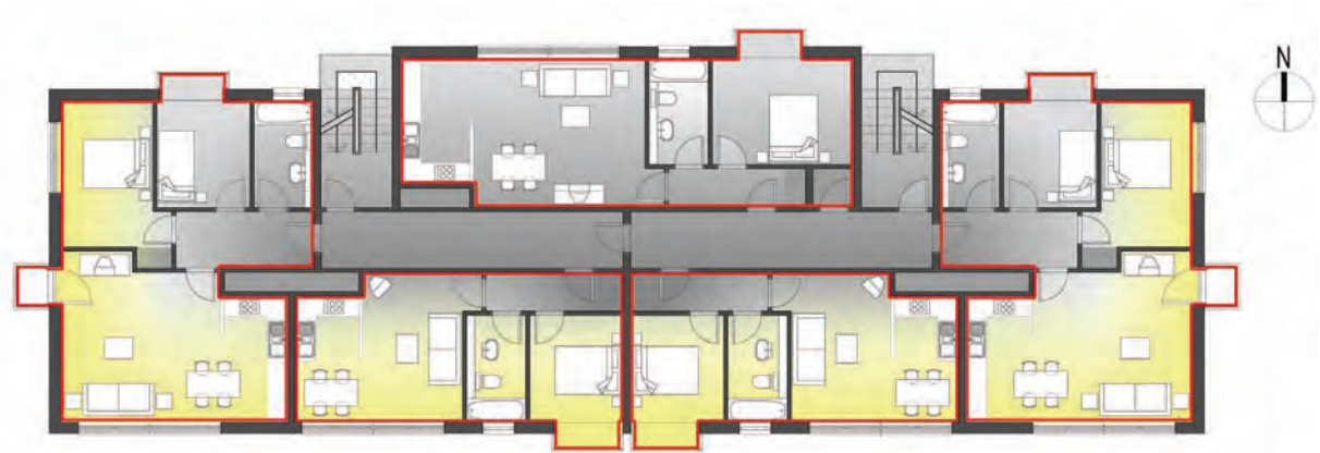
Figure 26: Careful layout design means that four out of the five flats shown have a south-facing living room
