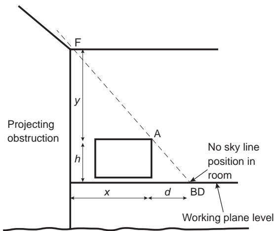
Figure D5: For a horizontal obstruction projecting from the window wall, the no sky line runs partly parallel to the obstruction and partly along a continuation of the line joining the end of the obstruction F and the side of the window A
