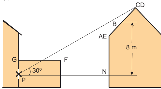
(a) Section
