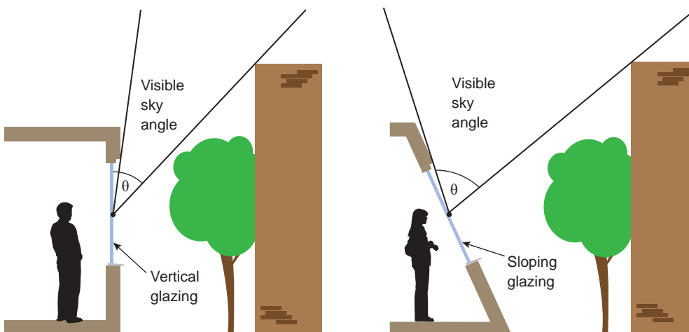
Figure 1: \theta is the angle of visible sky measured from the centre of the window, in a vertical plane (section) perpendicular to that of the window
